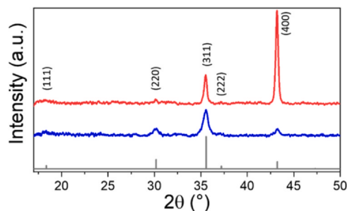
Fig. 2. \Theta - 2\theta X-ray diffraction patterns of CFO_30 (red), CFO_90 (blue) and CoFe 2 O 4 powder. Retrieved from the database JCPDS file #04-006-4148 [36].
